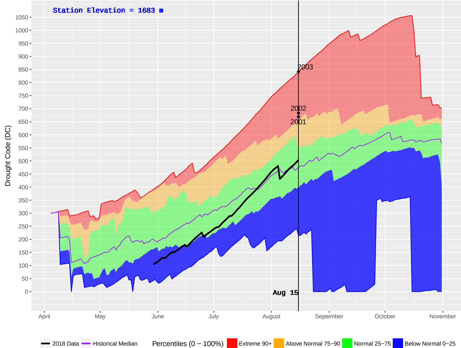
ASHNOLA (331) : Historical (1992–2016) and Current (2018) Daily Drought Code (DC)
