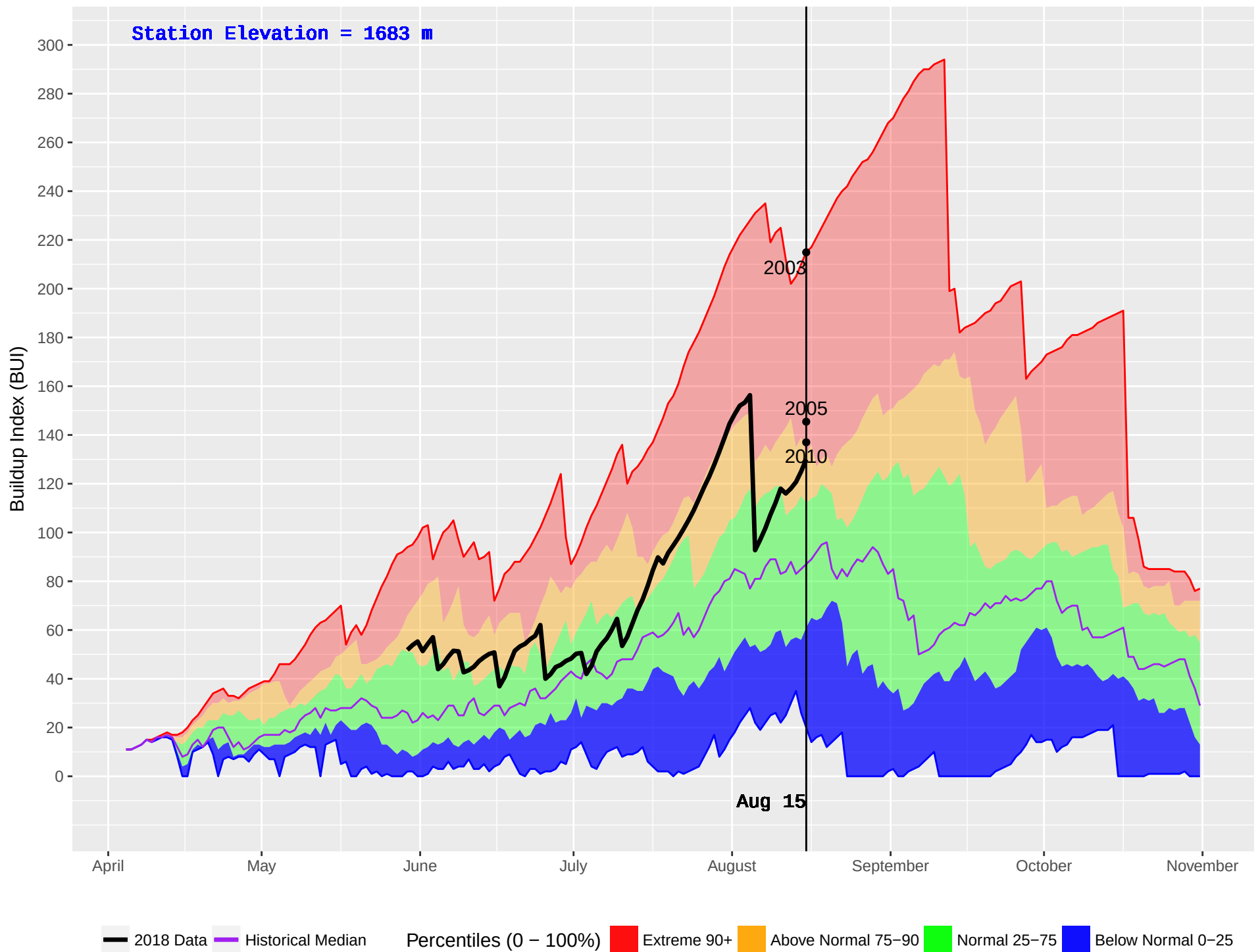
ASHNOLA (331) : Historical (1992–2016) and Current (2018) Daily Buildup Index (BUI)
